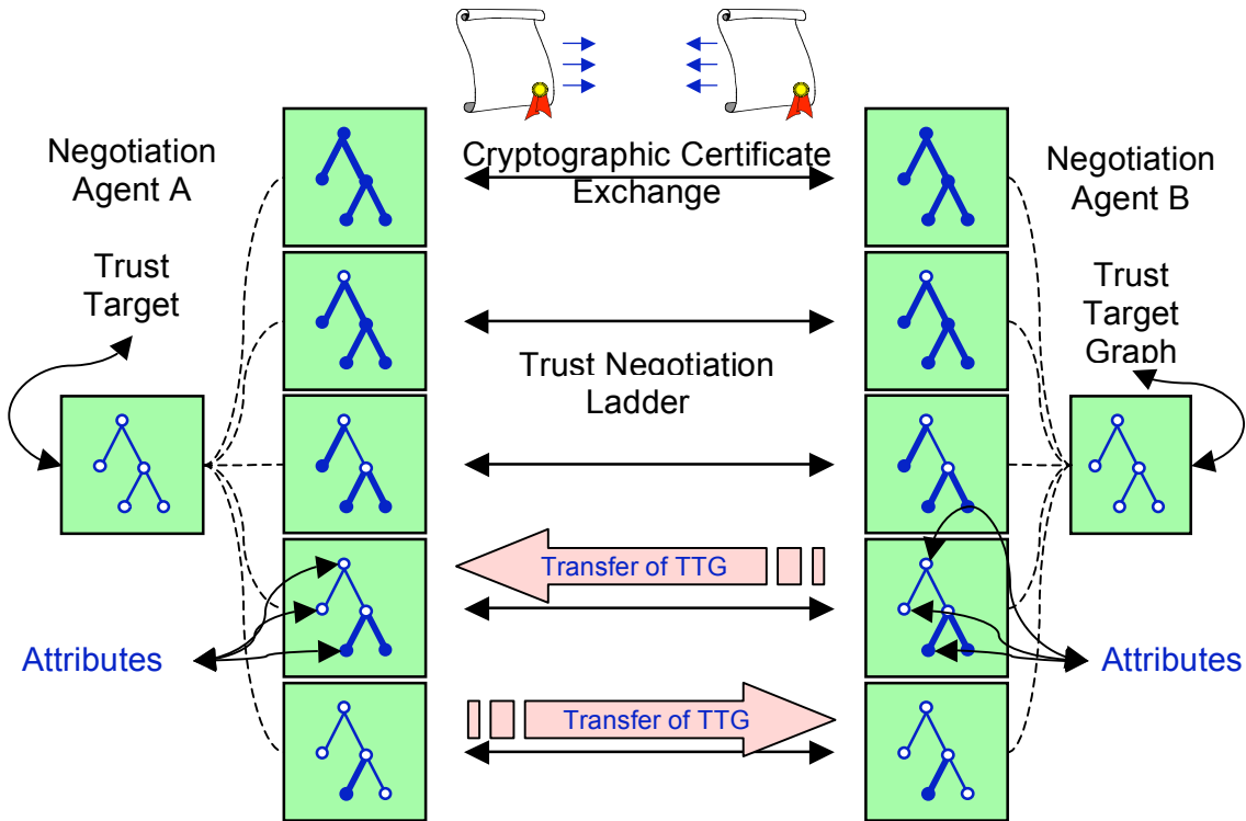
Figure 2: ABAC Trust Negotiation Overview
