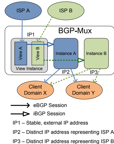
Figure 2: BGP-Mux Implementation
