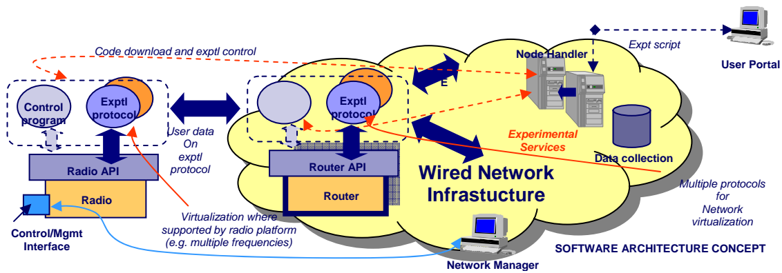
Figure 10 End-to-end software architecture
