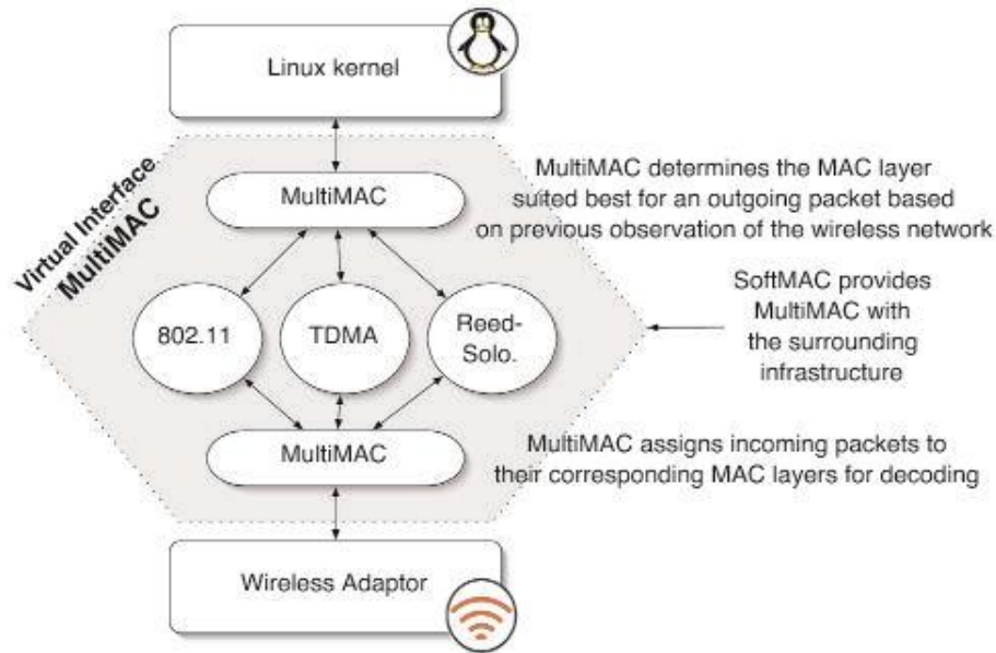
Fig 7. Architecture for virtualization of wireless MAC layer
