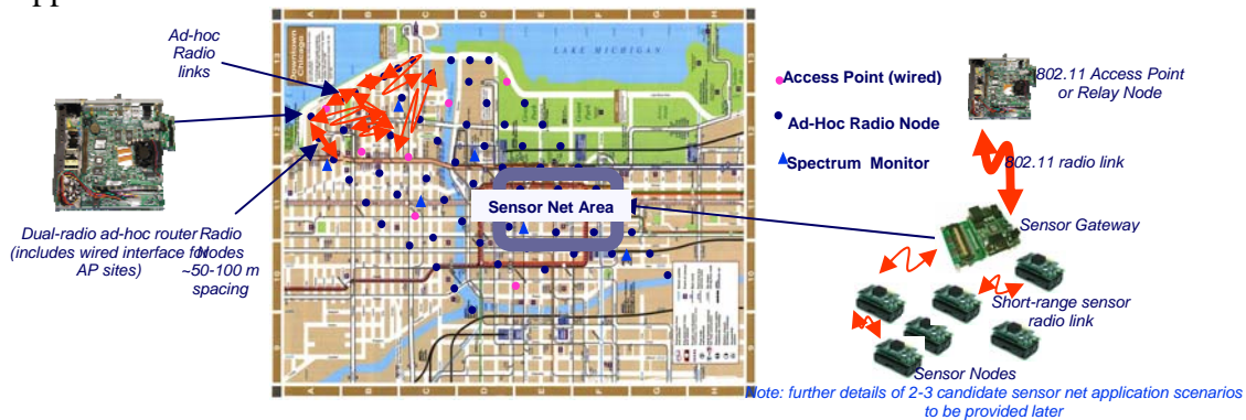
Figure 15 Deployment Concept for Sensor Networks
