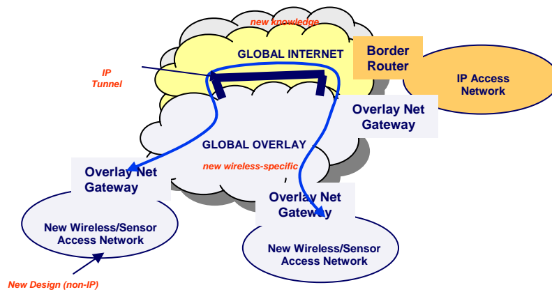
Fig. 3. Deployment of new wireless/sensor access network with overlay global backbone
