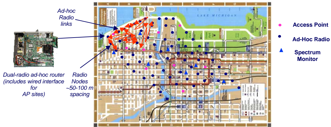
Figure 13 Deployment Concept for Ad-Hoc Mesh Network
