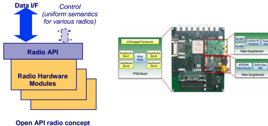
Figure 5 Open API Radio and Rice University Prototype
