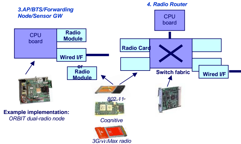
Figure 9 Radio Access Point/Forwarding Node and Radio Router Platforms
